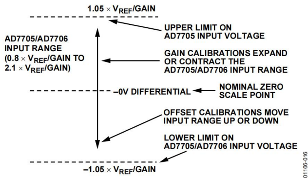
Figure 16. Span and Offset Limits
