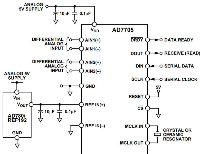
Figure 13. AD7705 Basic Connection Diagram
