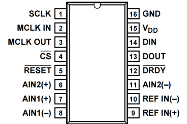
AD7705/AD7706 Pin Configuration
