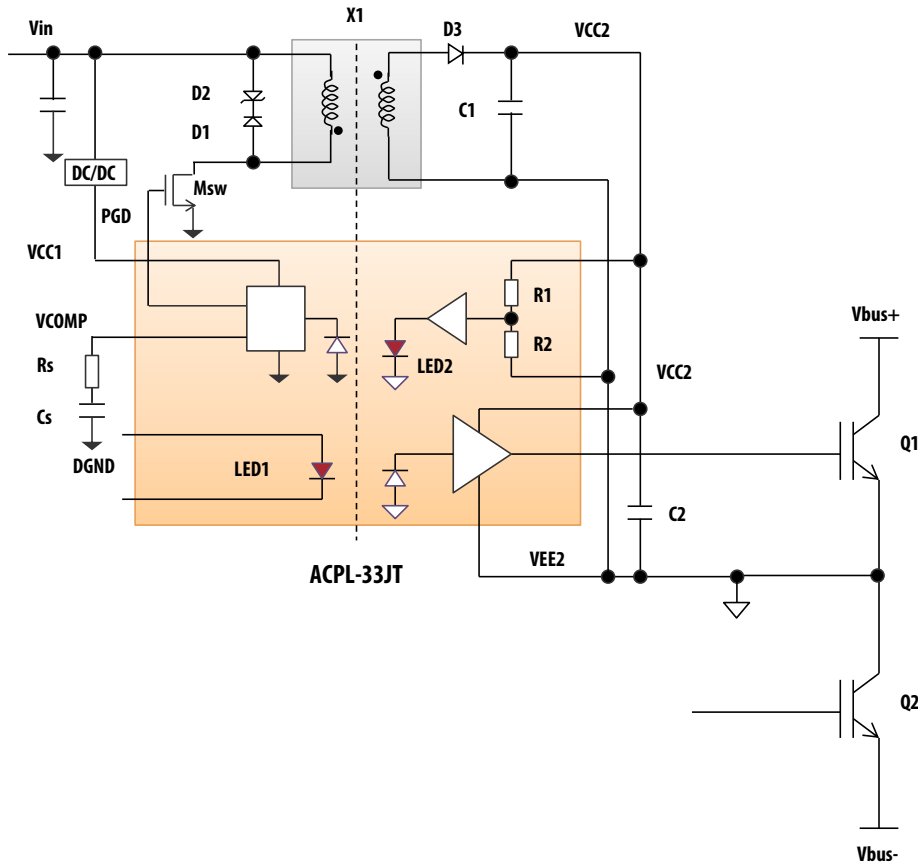
Figure 31 IGBT Gate Driver with Integrated Flyback Controller
