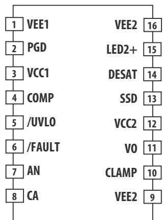
Figure 3 Pin out of ACPL-33JT
