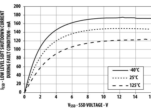
Figure 17 I_{SSD} vs. V_{SSD}
