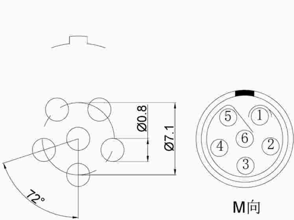
Pcb plate opening size (PCB板开孔尺寸)
