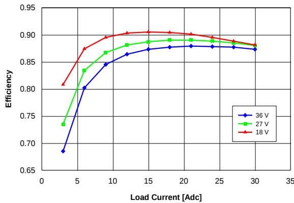
Figure 12. Efficiency vs. load current and input voltage for converter mounted vertically with air flowing from pin 3 to pin 1 at a rate of 300 LFM (1.5 m/s) and T_a = 25^\circ\text{C} .
