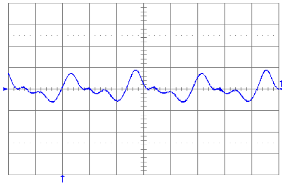
Figure 20. Output voltage ripple (20 mV/div.) at full rated load current into a resistive load with C_o = 10 F tantalum + 1 \mu F ceramic and V_{in} = 24 V. Time scale: 1 \mu s/div...
