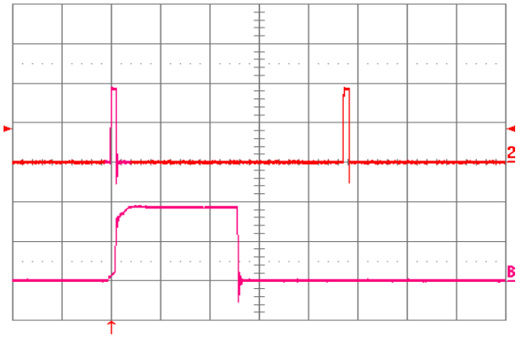
Figure 25. Load current (top trace, 20 A/div, 20 ms/div) into a 10 m \Omega short circuit during restart, at V_{in} = 24 V. Bottom trace (20 A/div, 1 ms/div) is an expansion of the on-time portion of the top trace..
