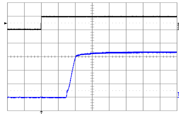
Figure 16. Turn-on transient at full rated load current (resistive) with no out-put capacitor at V_{in} = 24\text{ V} , triggered via ON/OFF pin. Top trace: ON/OFF signal (5 V/div.). Bottom trace: output voltage (1 V/div.). Time scale: 1 ms/div.
