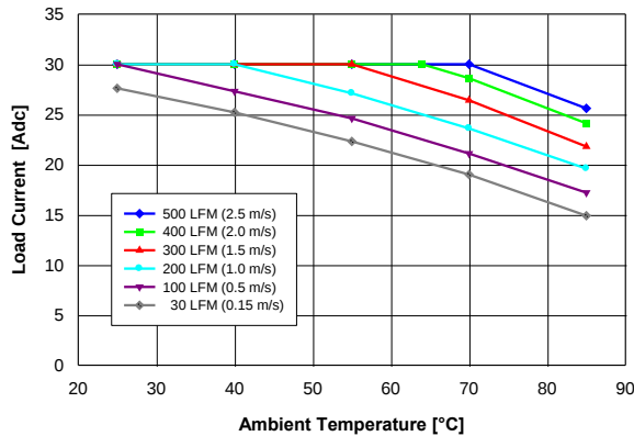
Figure 8. Available load current vs. ambient air temperature and airflow rates for converter mounted vertically with V_{in} = 27 V, air flowing from pin 3 to pin 1 and maximum FET temperature \leq 120 °C.
