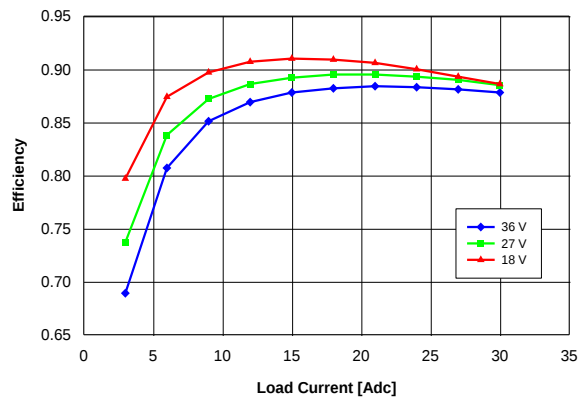
Figure 14. Efficiency vs. load current and input voltage for converter mounted horizontally with air flowing from pin 3 to pin 4 at a rate of 300 LFM (1.5 m/s) and T_a = 25^\circ\text{C} .
