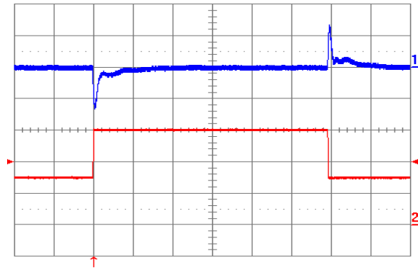
Figure 19. Output voltage response to load current step-change (7.5 A – 15 A – 7.5 A) at V_{in} = 24 V. Top trace: output voltage (100 mV/div.). Bottom trace: load current (5 A/div.). Current slew rate: 5 A/ \mu s. C_o = 450 \mu F tantalum + 1 \mu F ceramic. Time scale: 0.2 ms/div.
