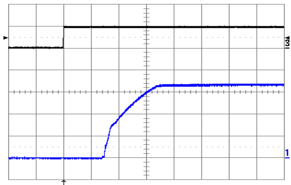
Figure 17. Turn-on transient at full rated load current (resistive) plus 10,000 F at V_{in} = 24\text{ V} , triggered via ON/OFF pin. Top trace: ON/OFF signal (5 V/div.). Bottom trace: output voltage (1 V/div.). Time scale: 1 ms/div.
