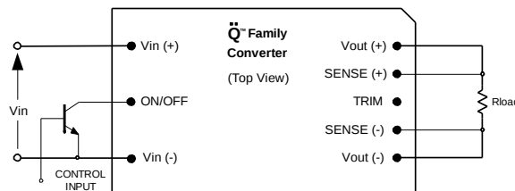
Figure 1. Circuit configuration for ON/OFF function.
