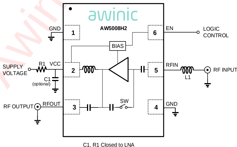
Figure 1 Typical Application Circuit of AW5008H2
