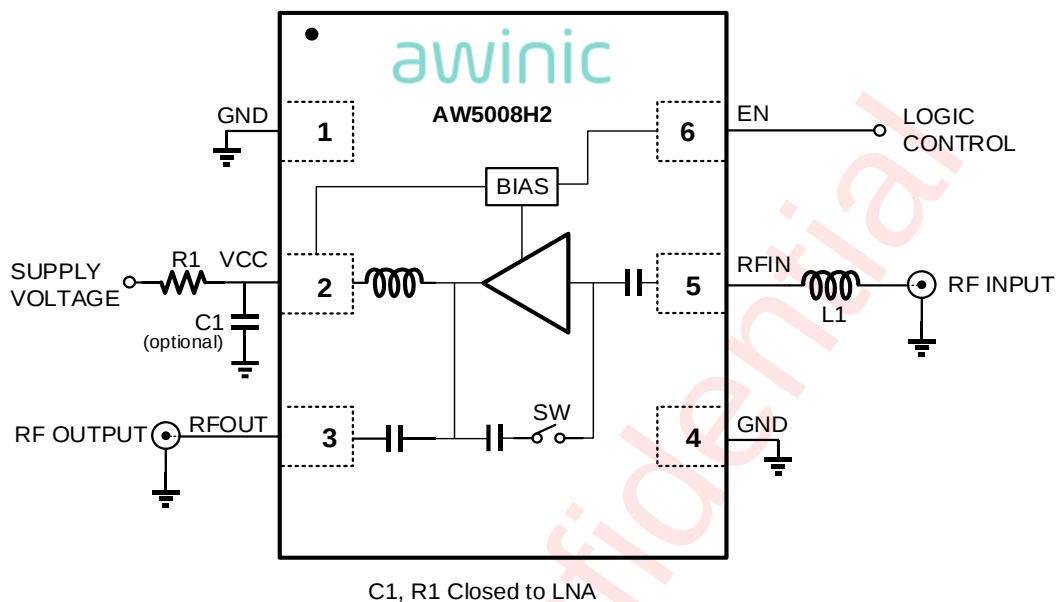
Figure 4 AW5008H2 DC Test Diagram
