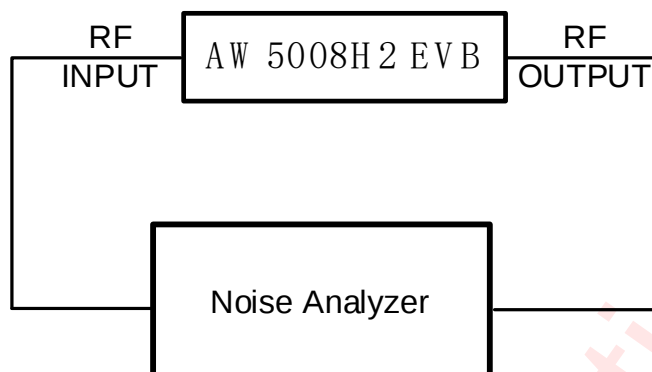
Figure 6 AW5008H2 Noise Figure Measurement Diagram
