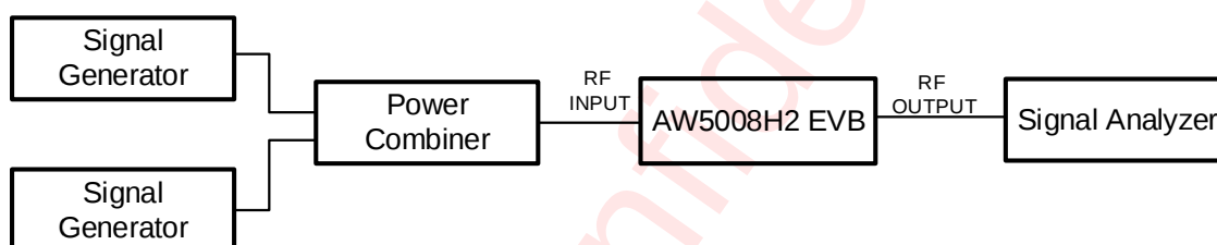
Figure 7 AW5008H2 IIP3 Measurement Diagram
