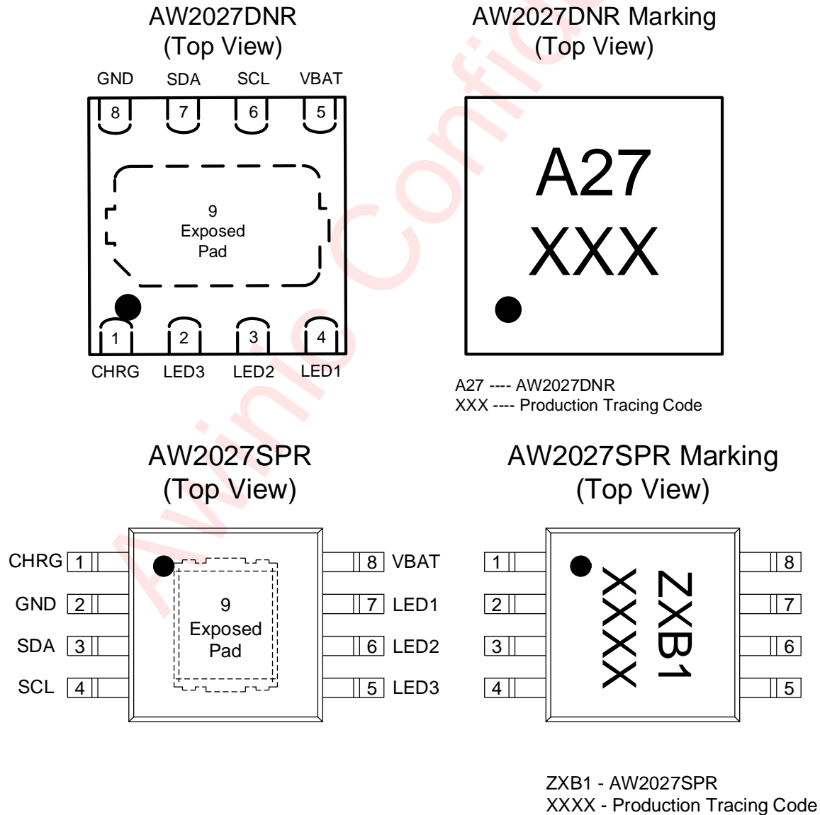
Figure 1 Pin Configuration and Top Marking
