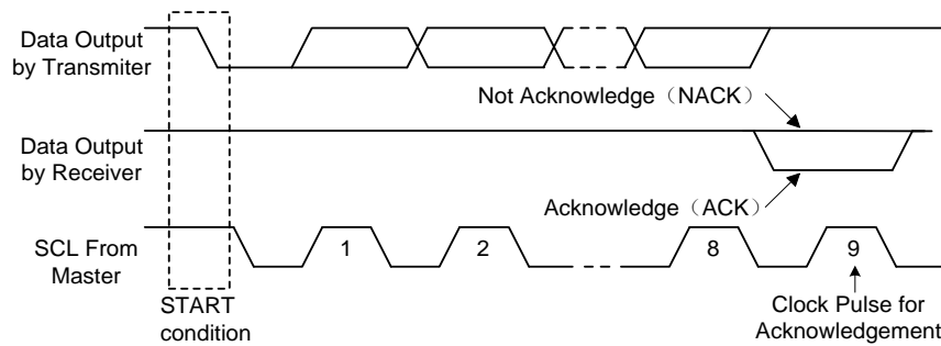
Figure 9 I²C ACK Timing
