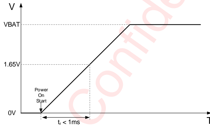
Figure 5 AW2027 Power on Timing
