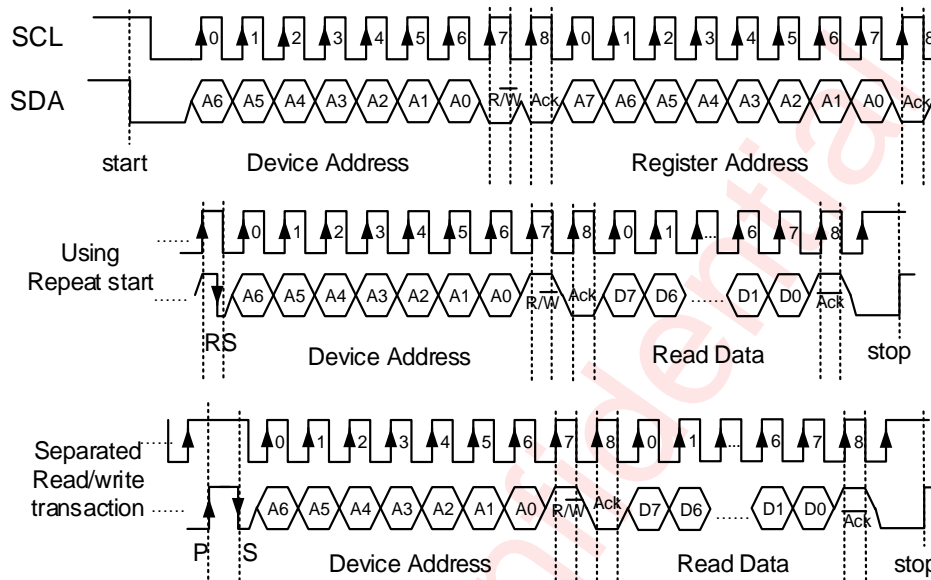
Figure 11 I 2 C Read Byte Cycle
