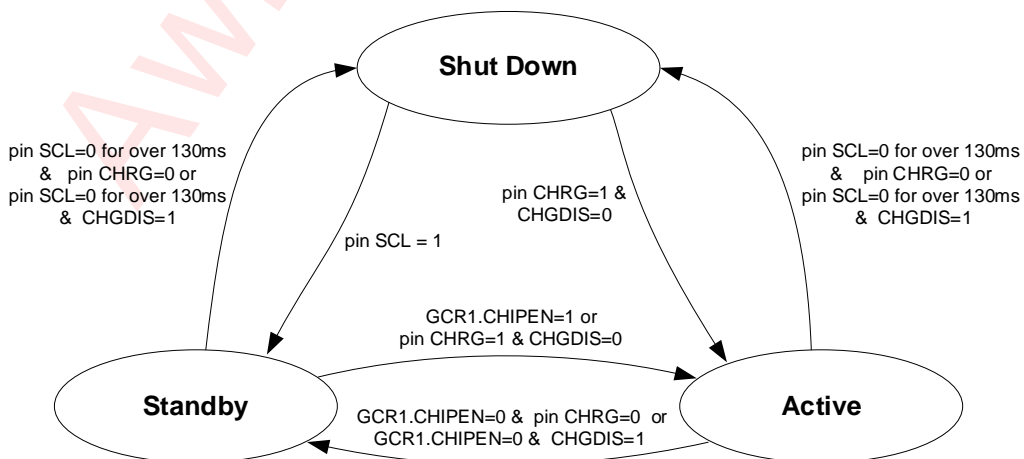
Figure 6 AW2027 Operating Modes Transition
