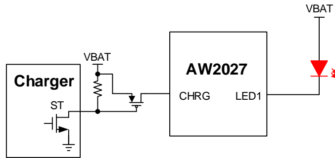
Figure 15 Real Charging Status Indication in Special Charger IC Application
