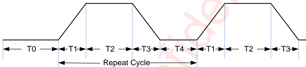
Figure 12 LED Breath Timing in Pattern Mode
