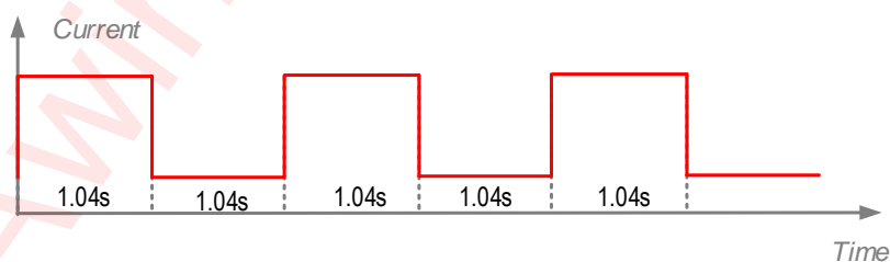
Figure 14 Blinking Waveform on LED1 for Auto Charging Indication
