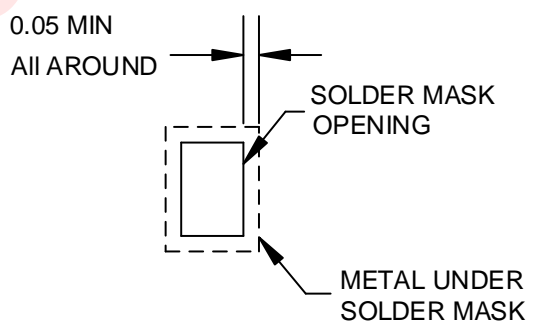
SOLDER MASK DEFINED
