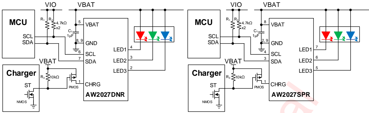
Charging Status Indication Application
