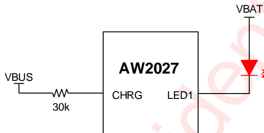
Figure 16 USB Power Insertion Status Indication in PMU-Controlled Charging Application
