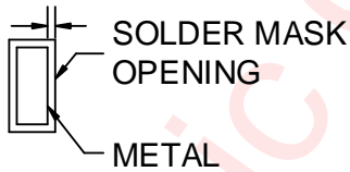
NON-SOLDER MASK DEFINED
