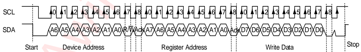
Figure 10 I²C Write Byte Cycle
