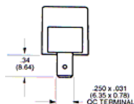
5 - Quick Connect .250"
