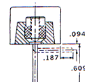
GBPNX .062" Dia 90Degree printed circuit pin
