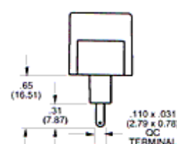
3 - Quick Connect .110
