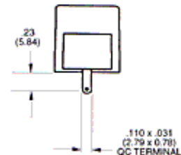
3 - Quick Connect .110"
