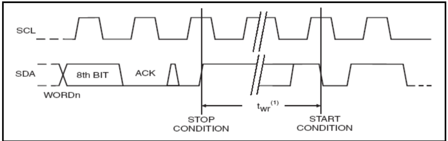
Figure 11. SCL: Serial Clock, SDA: Serial Data I/O
