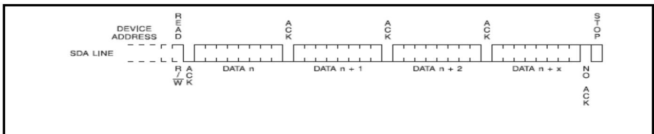
Figure 9. Sequential Read
