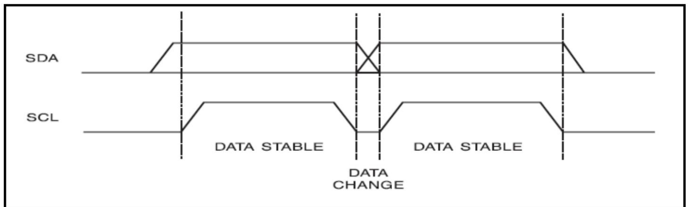
Figure 1. Data Validity
