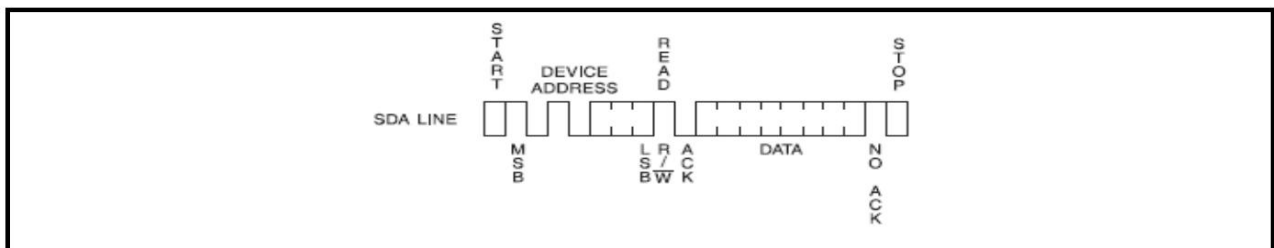
Figure 8. Random Read
