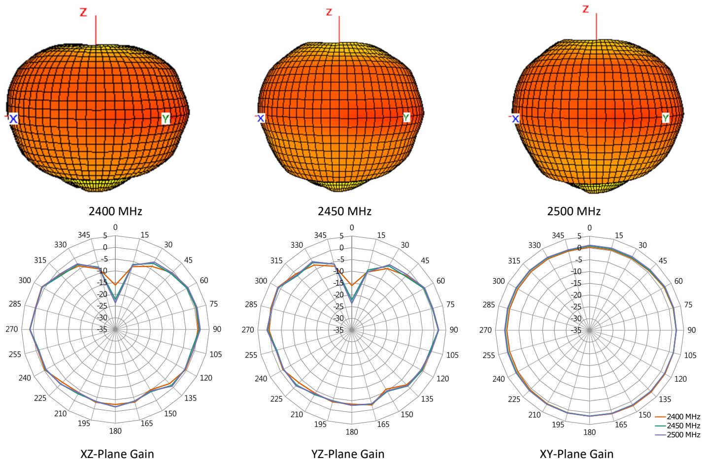
Figure 10. Antenna Radiation Patterns, Straight without ground plane
