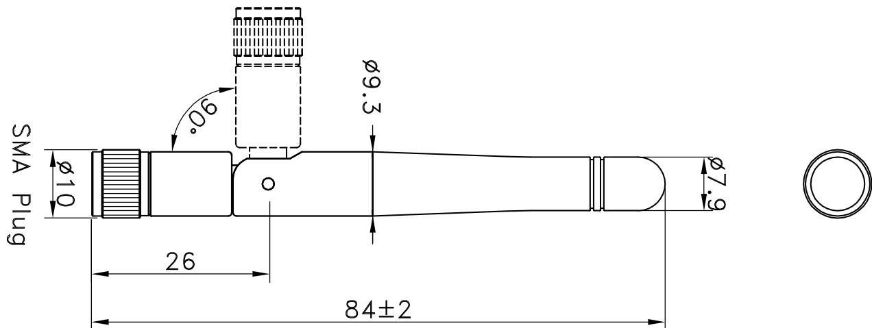
Figure 2. Antenna Dimensions
