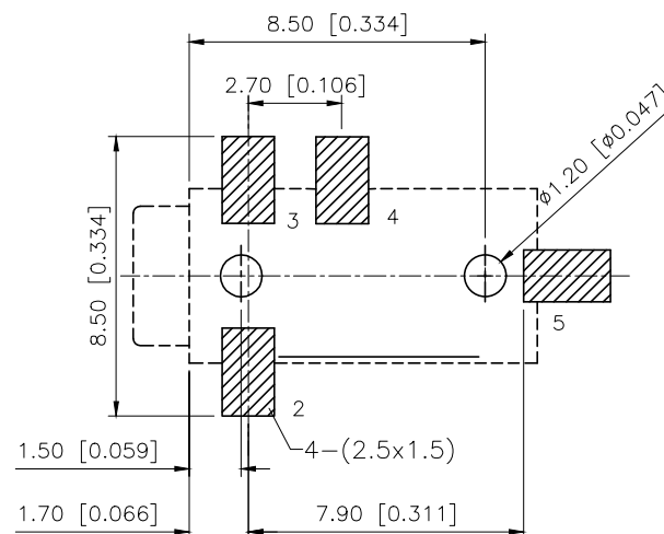
T:1.6 Dimensions of PC board holes Tolerance :±0.1(Printed-sided view)
