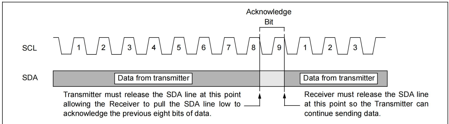
FIGURE 4-2: ACKNOWLEDGE TIMING
