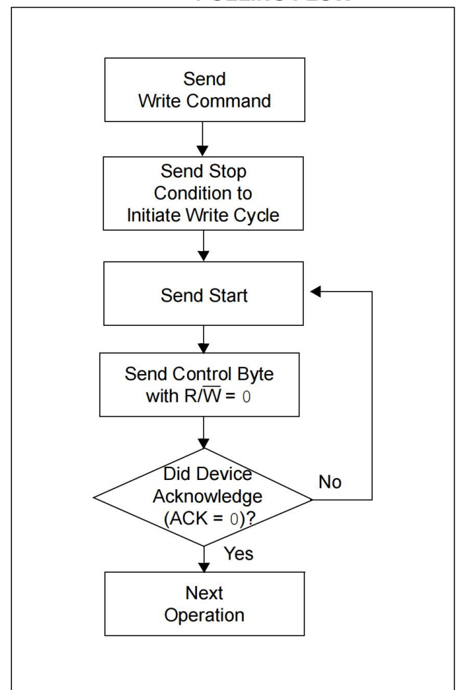
FIGURE 7-1: ACKNOWLEDGE POLLING FLOW
