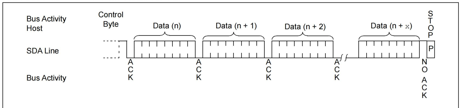
FIGURE 8-3: SEQUENTIAL READ
