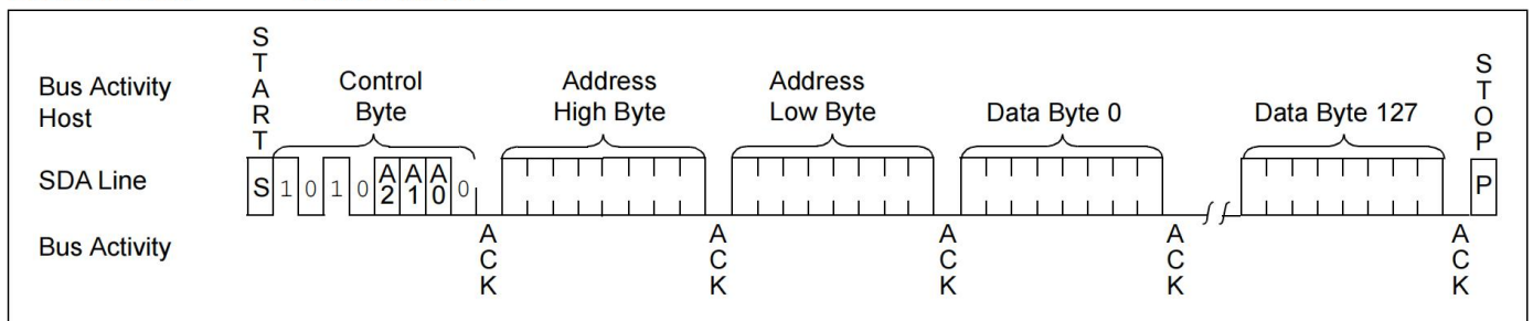
FIGURE 6-2: PAGE WRITE
