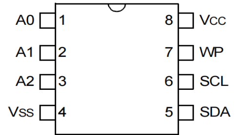
8-Lead PDIP/SOIC (Top View)
