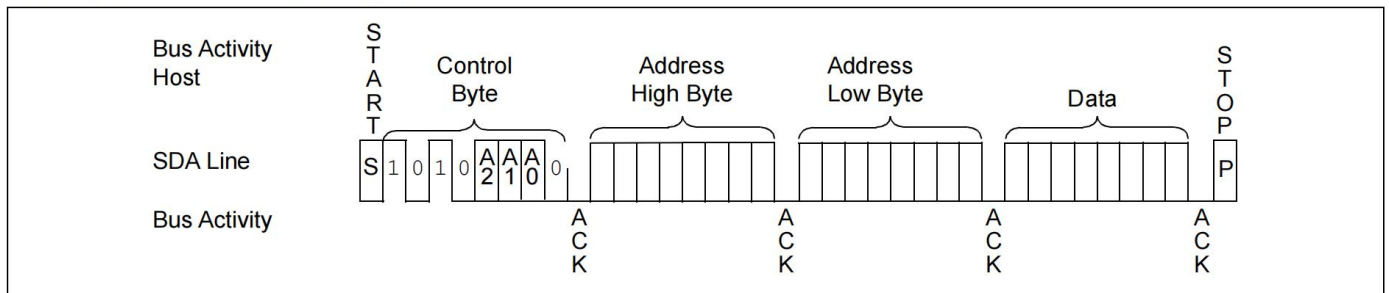
FIGURE 6-1: BYTE WRITE
