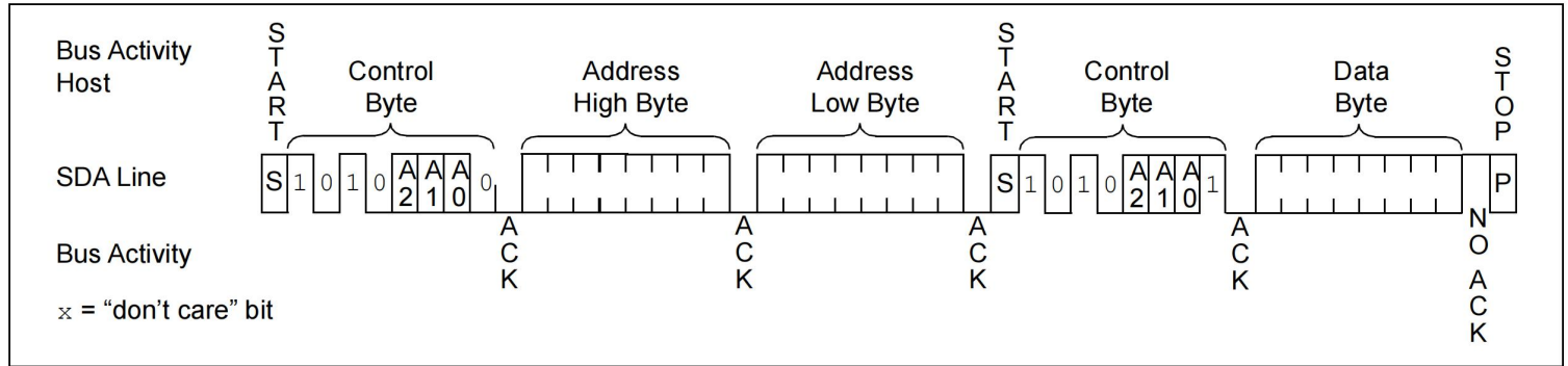
FIGURE 8-2: RANDOM READ
