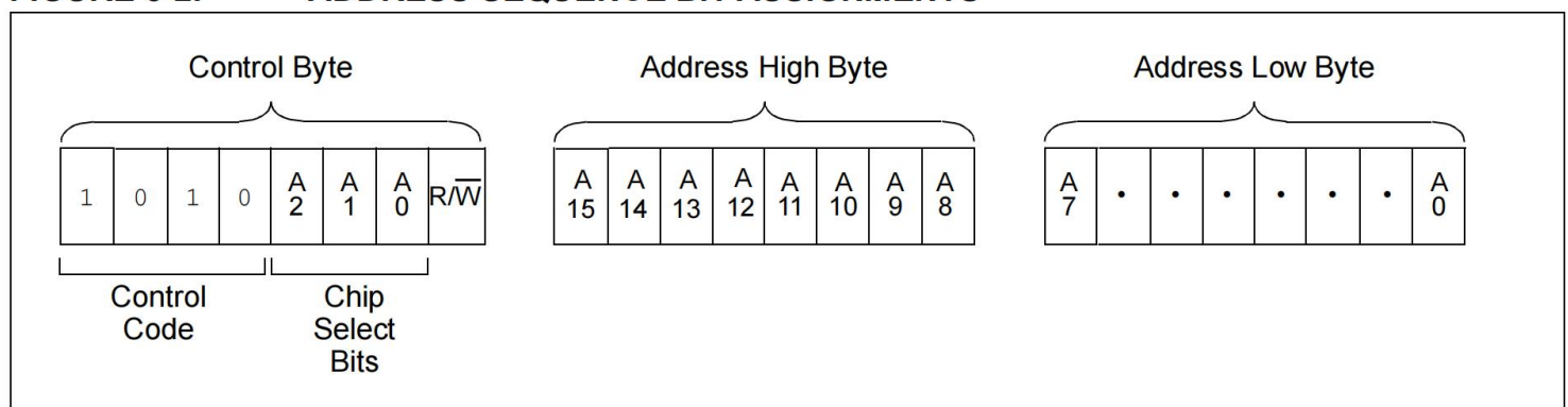
FIGURE 5-2: ADDRESS SEQUENCE BIT ASSIGNMENTS
