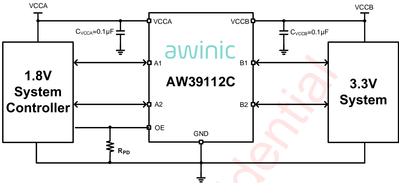
Figure 1 Typical Application Circuit of AW39112C
