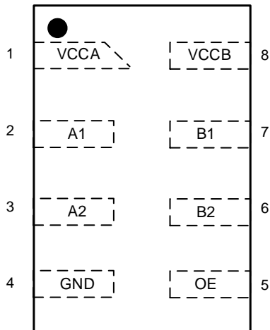
AW39112CDNR PIN Configuration (Top View)
