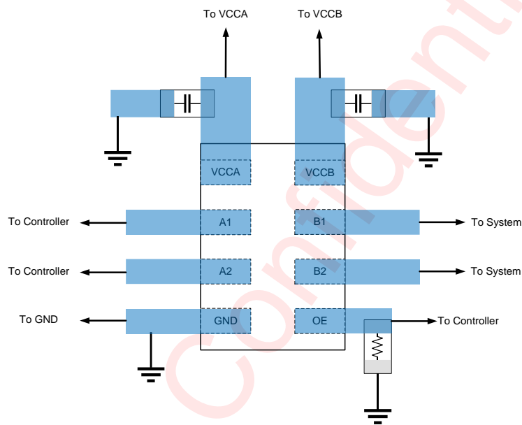
Figure 15 AW39112CDNR Layout Example
