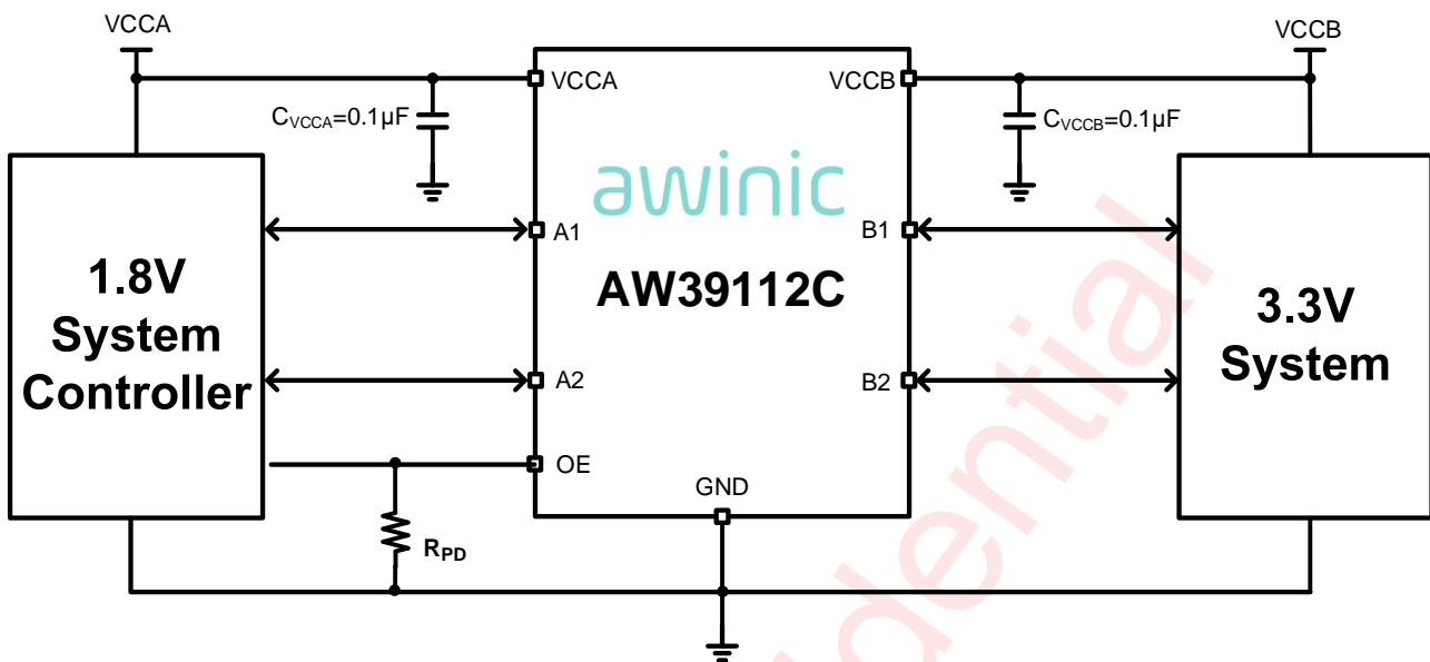
Figure 14 AW39112C Application Circuit
