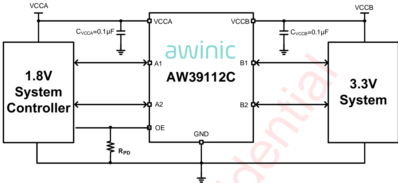
Figure 4 AW39112C Application Circuit
