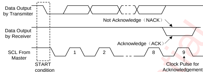
I 2 C ACK Timing
