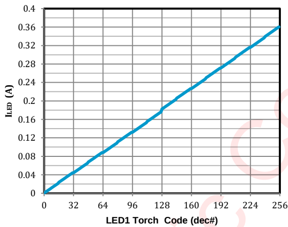
LED1 Torch Current vs Brightness Code
