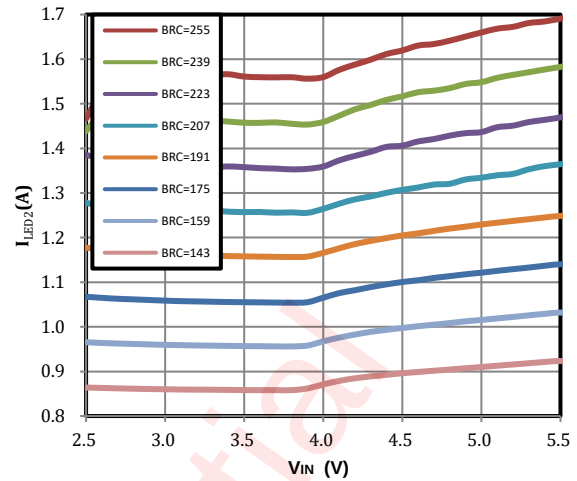
LED2 Flash Current vs Input Voltage
