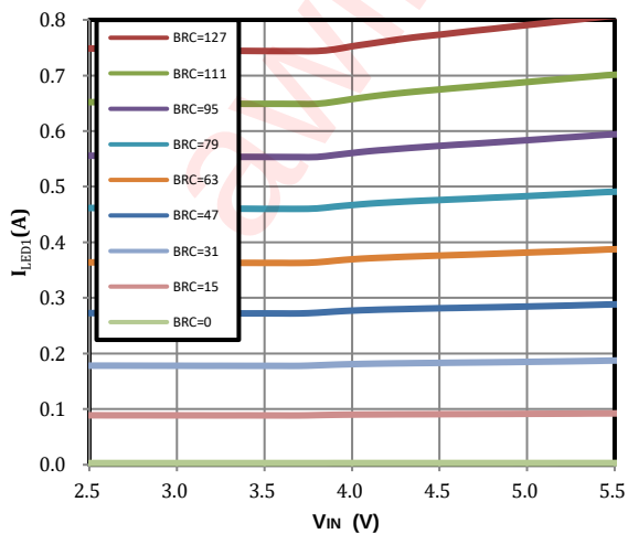
LED1 Flash Current vs Input Voltage
