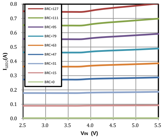
LED2 Flash Current vs Input Voltage
