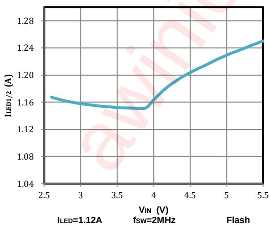
LED1/2 Flash Current vs Input Voltage
