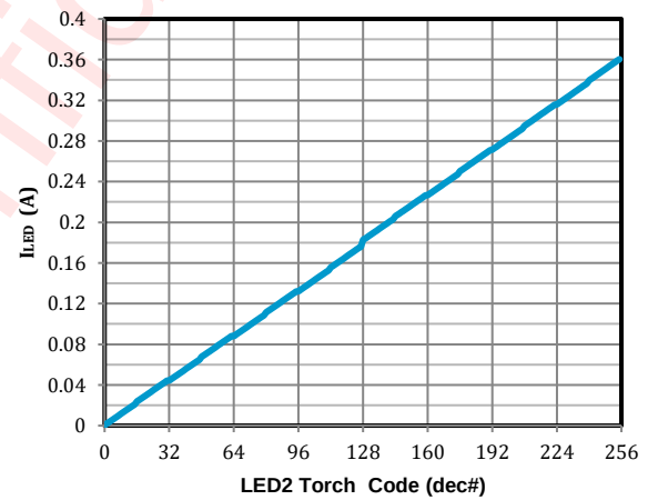
LED2 Torch Current vs Brightness Code
