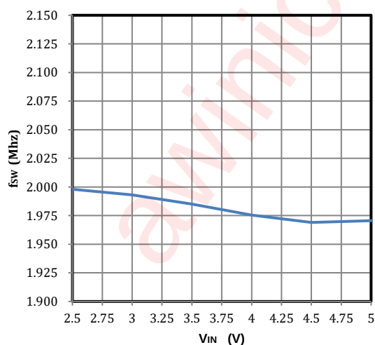
2-MHz Frequency vs Input Voltage
