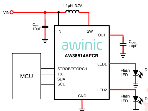
AW36514A Application Circuit
