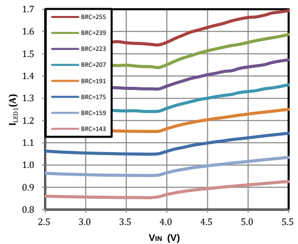
LED2 Flash Current vs Input Voltage
