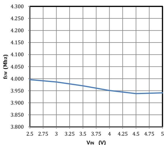
4-MHz Frequency vs Input Voltage
