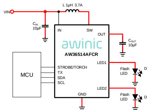
Typical Application Circuit of AW36514A
