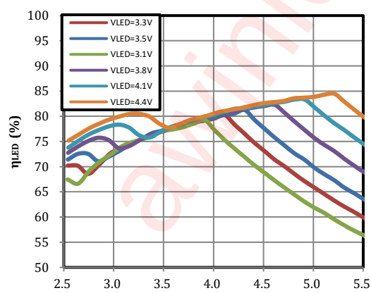
LED Efficiency vs Input Voltage
