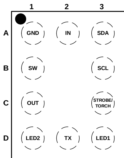
AW36514AFCR Pin Configuration (Top View)
