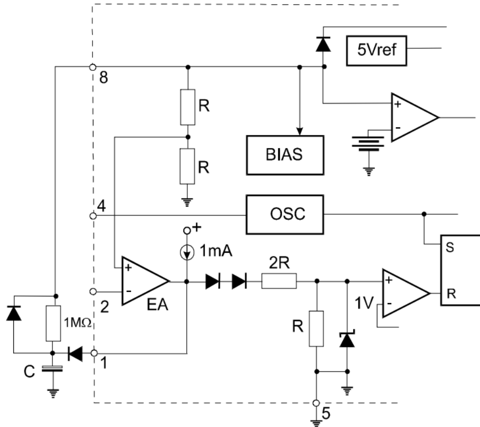
Figure 8. Soft-Start Circuit
