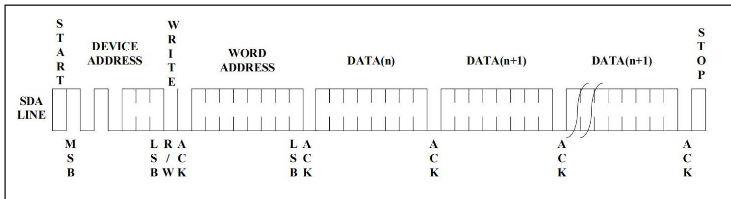
Figure 7. Page Write
