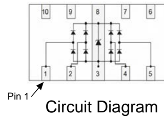
DFN2510-10L ( UDFN-10(1x2.5))
