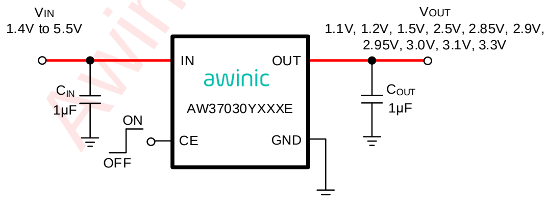
AW37030YXXxE Application Circuit
