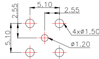
PCB.WELDING DRAWING (TOLERANCE:±0.05)
