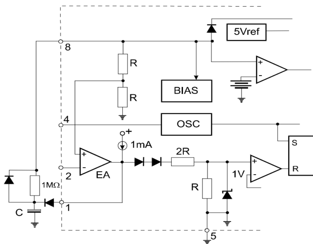
Figure 8. Soft-Start Circuit
