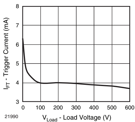
Fig. 11 - Trigger Current vs. Load Voltage
