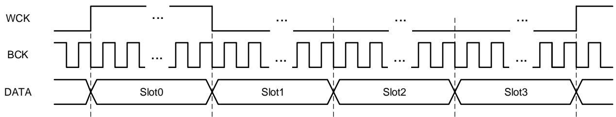
Figure 13 TDM Timing
