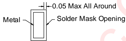
Non-solder Mask Defined
