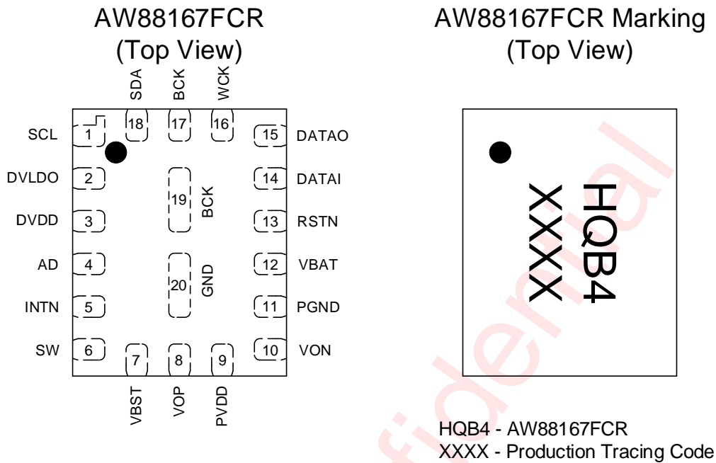
Figure 1 AW88167FCR pin diagram top view and device marking
