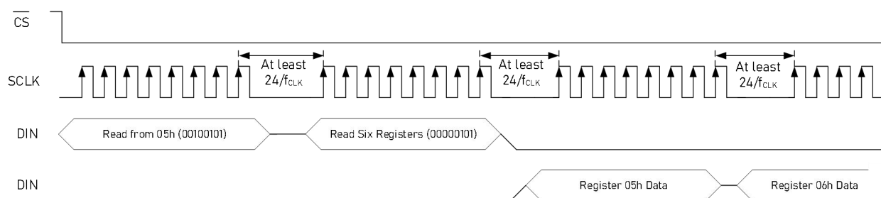
Fig. 34 RREG Sequence
