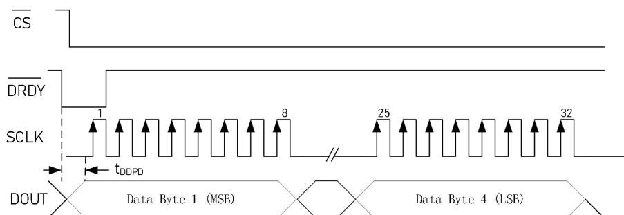
Fig. 30 Read-data-continuous Timing
