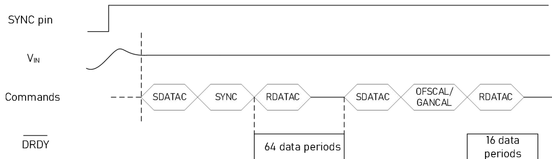
Fig. 32 Calibration Timing
