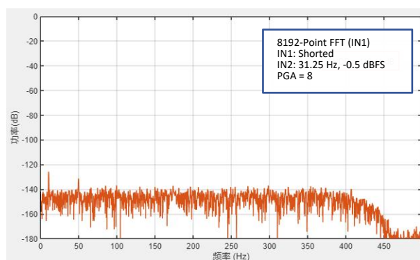
Fig. 18 Crosstalk Spectrum
