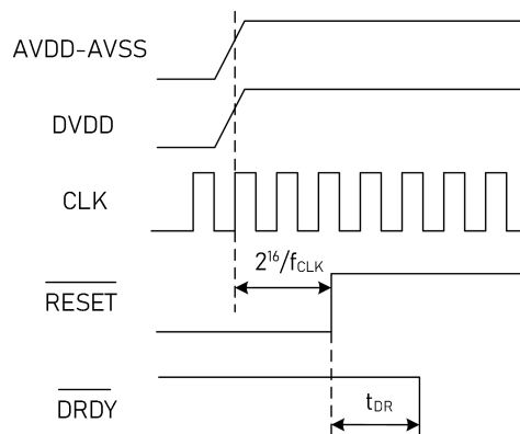
Fig. 29 Power-on Sequence
