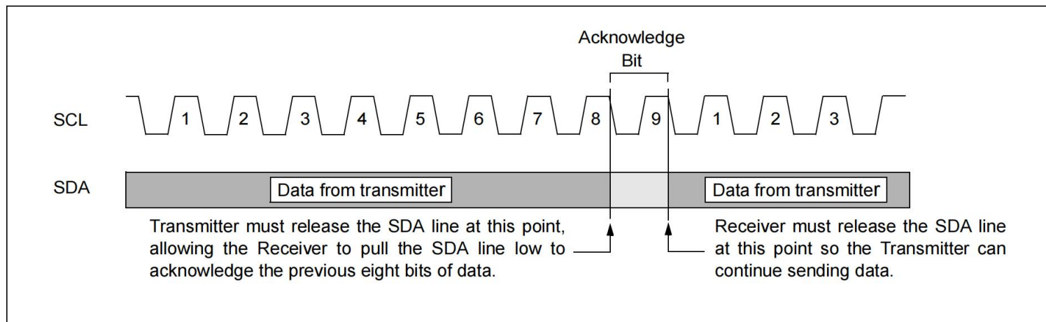
FIGURE 4-2: ACKNOWLEDGE TIMING
