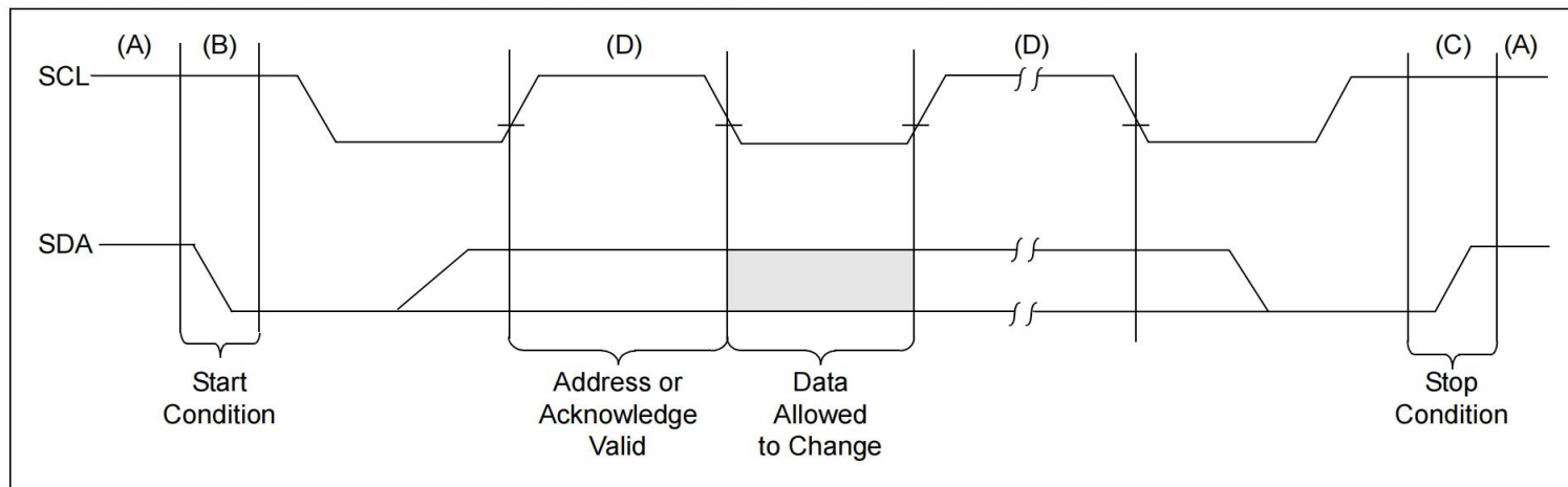
FIGURE 4-1: DATA TRANSFER SEQUENCE ON THE SERIAL BUS
