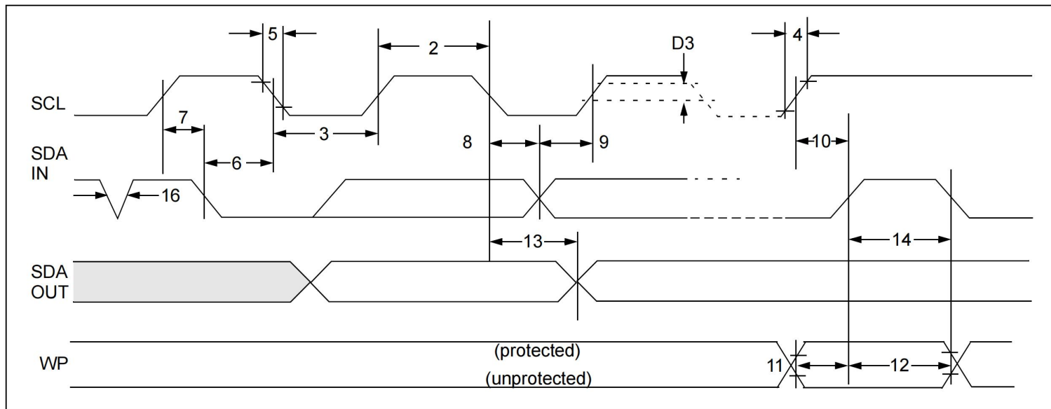
FIGURE 1-1: BUS TIMING DATA
