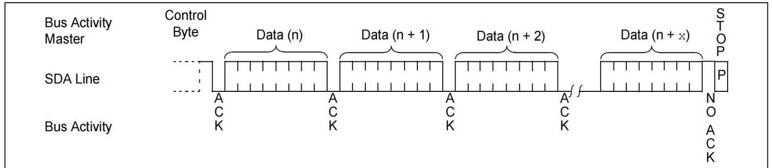
FIGURE 8-3: SEQUENTIAL READ
