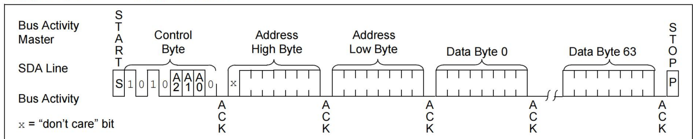
FIGURE 6-2: PAGE WRITE
