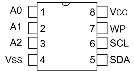
8-Lead PDIP (Top View)
