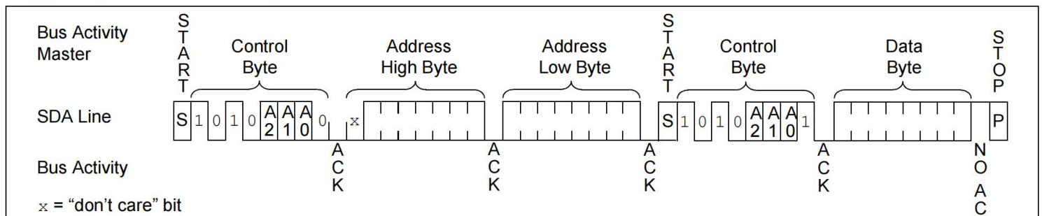
FIGURE 8-2: RANDOM READ
