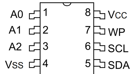
8-Lead SOIC/TSSOP (Top View)
