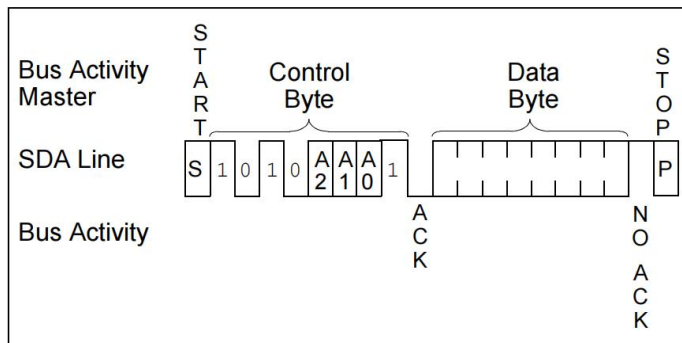
FIGURE 8-1: CURRENT ADDRESS READ
