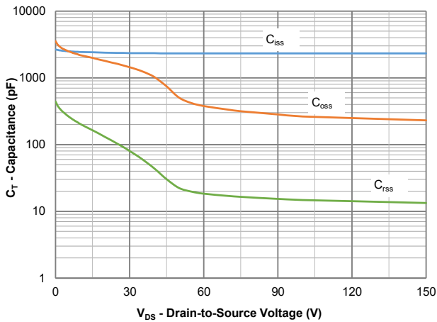
Figure 9: Capacitance Characteristics
