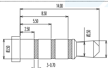
Ø3.50mm 4 POLE PLUG DETAIL
