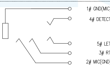
SCHEMATIC
