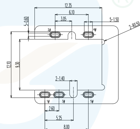
PCB LAYOUT (TOP VIEW) TOLERANCE: ±0.05
