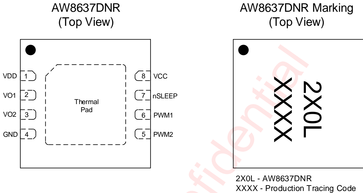
Figure 1 Pin Configuration And Top Mark
