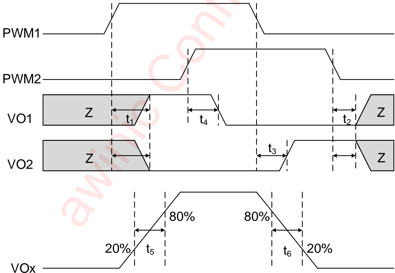
Figure 4 Input and Output Timing for AW8637
