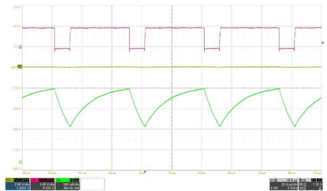
Figure 6 80% Duty Cycle Reverse Direction
