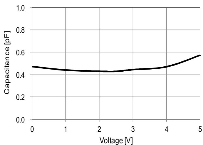
Voltage—Capacitance Characteristic
