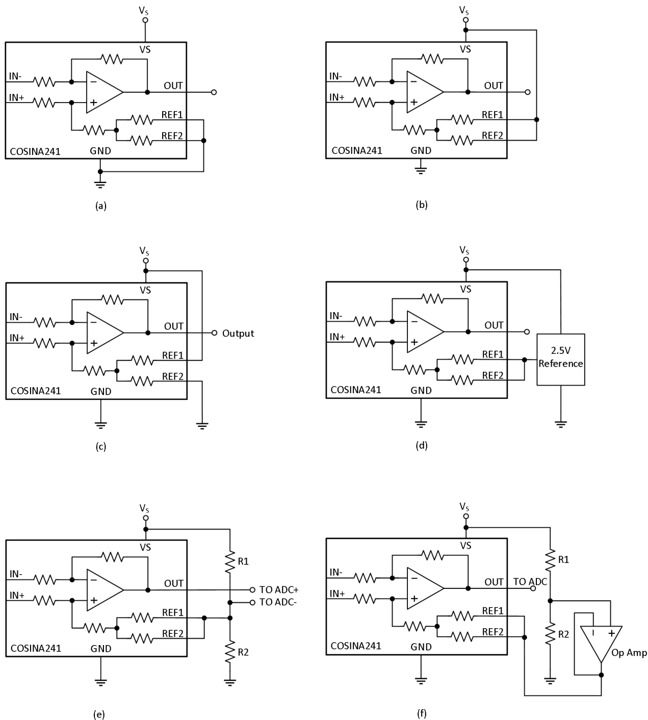
Figure 3 Adjusting the Output with the Reference Pins
