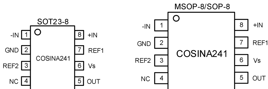
Figure 1 Pin Diagram
