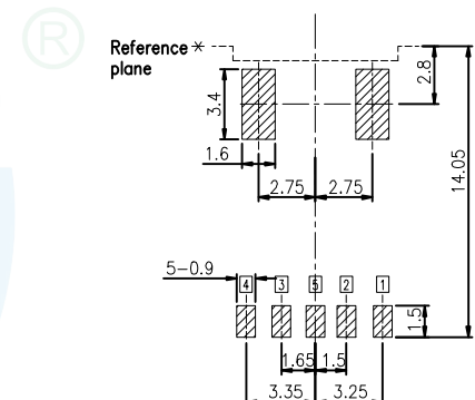
Recommended PCB Layout Tolerance: ±0.1(Top view)
