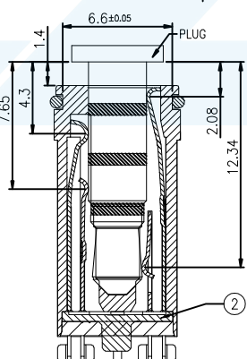
SEC:A-A Image of plug match with contact point
