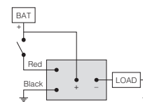
High side switching application
