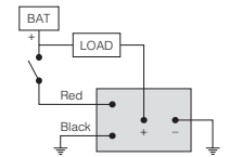
Low side switching application
