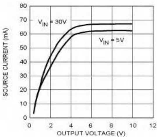
Source Current vs. Output Voltage
