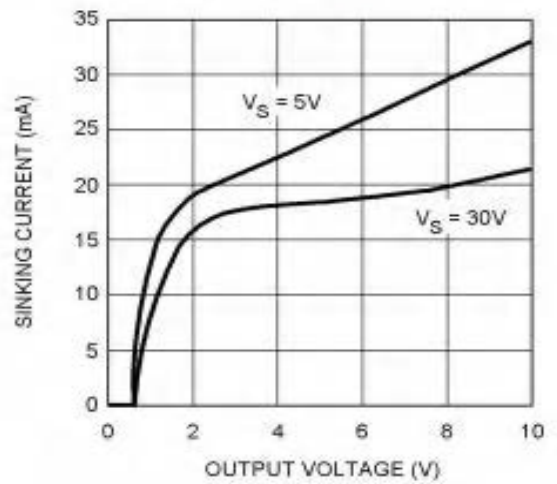
Sinking Current vs. Output Voltage
