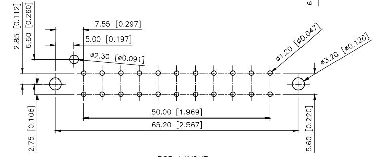
PCB LAYOUT
