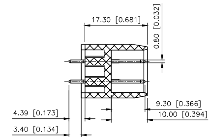
SECTION:A-A SCALE:1:1
