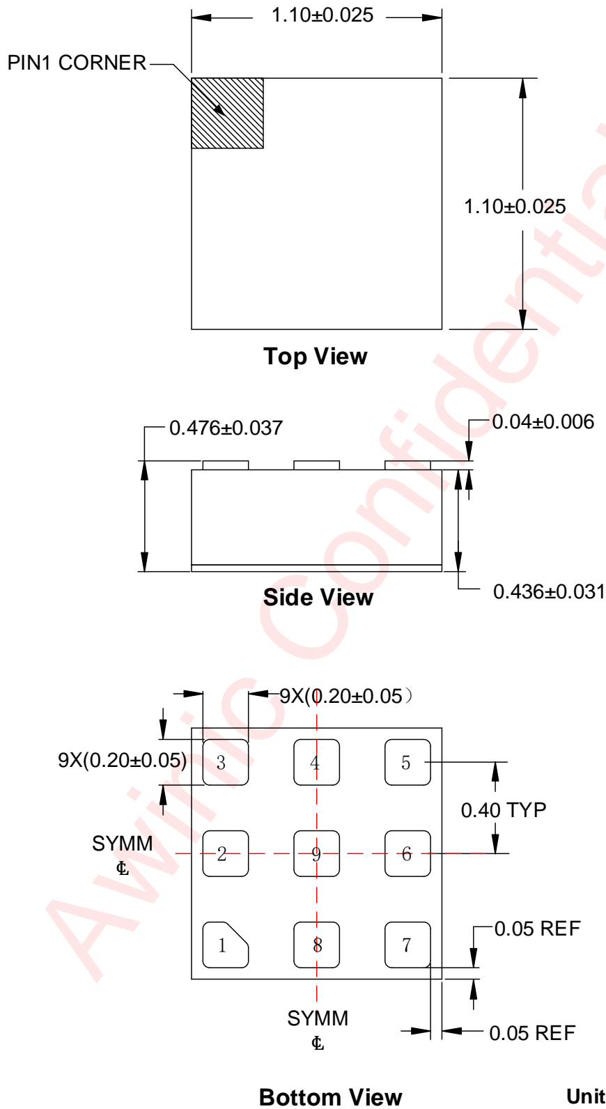
Figure 15 Package Outline
