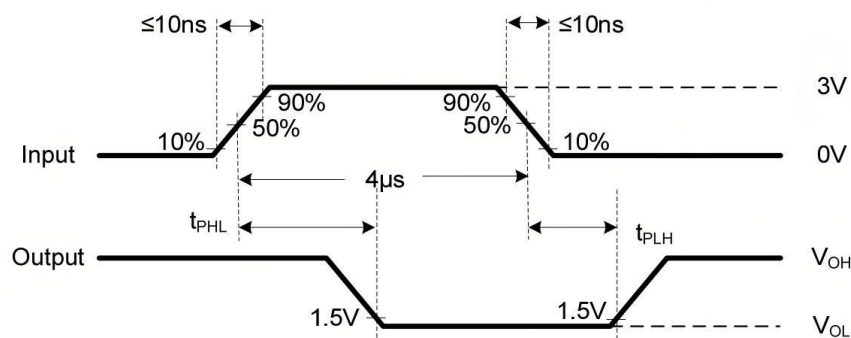
Receiver Waveforms
