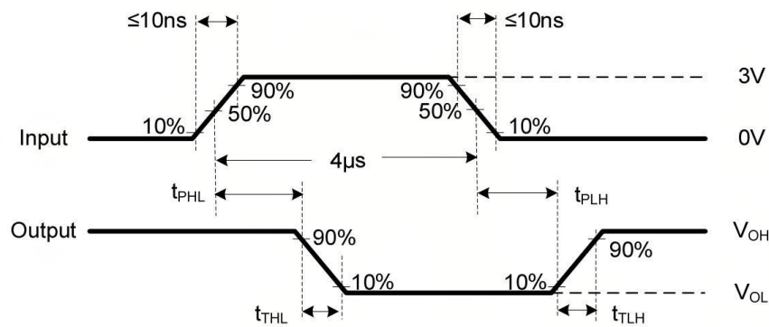
Transmitter Waveforms
