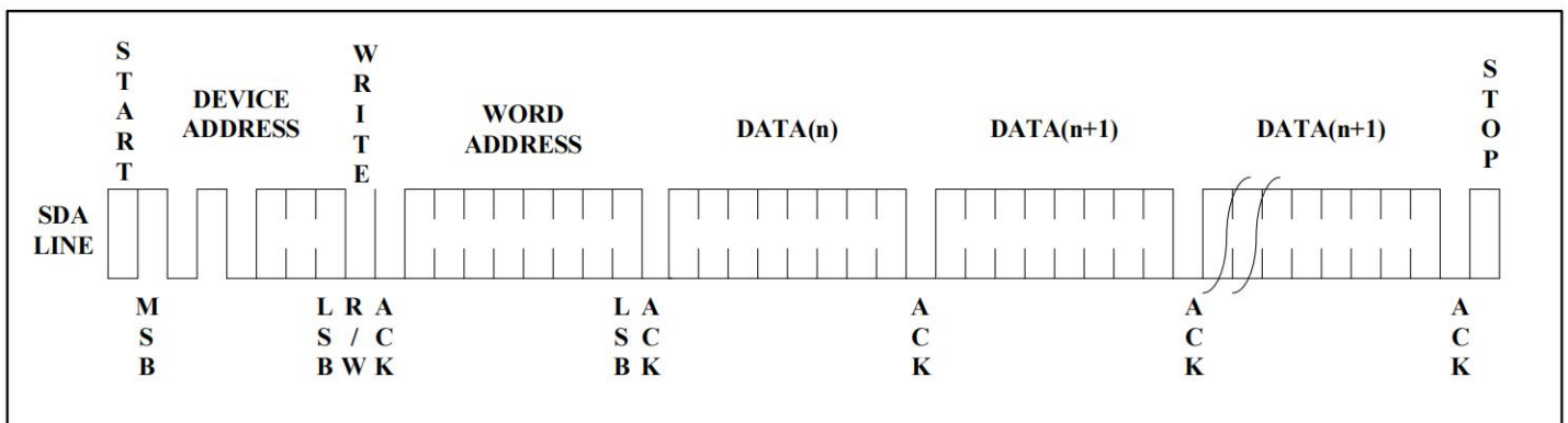
Figure 7. Page Write
