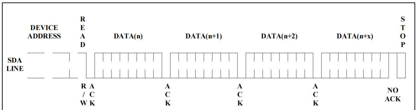
Figure 10. Sequential Read
