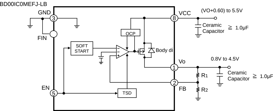
Figure 1. Block Diagram
