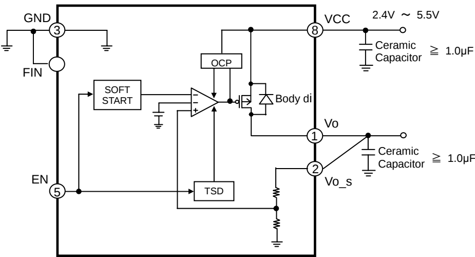
Figure 2. Block Diagram (Fixed type)
