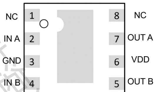
SOP-8
