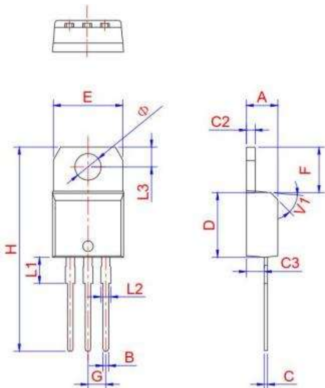
TO-220B Non-Ins
