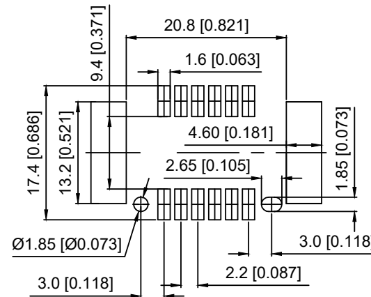
PCB Layout
