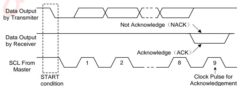
Fig 26 Acknowledgement Diagram
