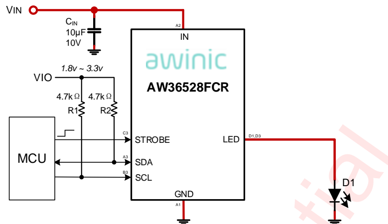
Fig 3 AW36528 Application Circuit
