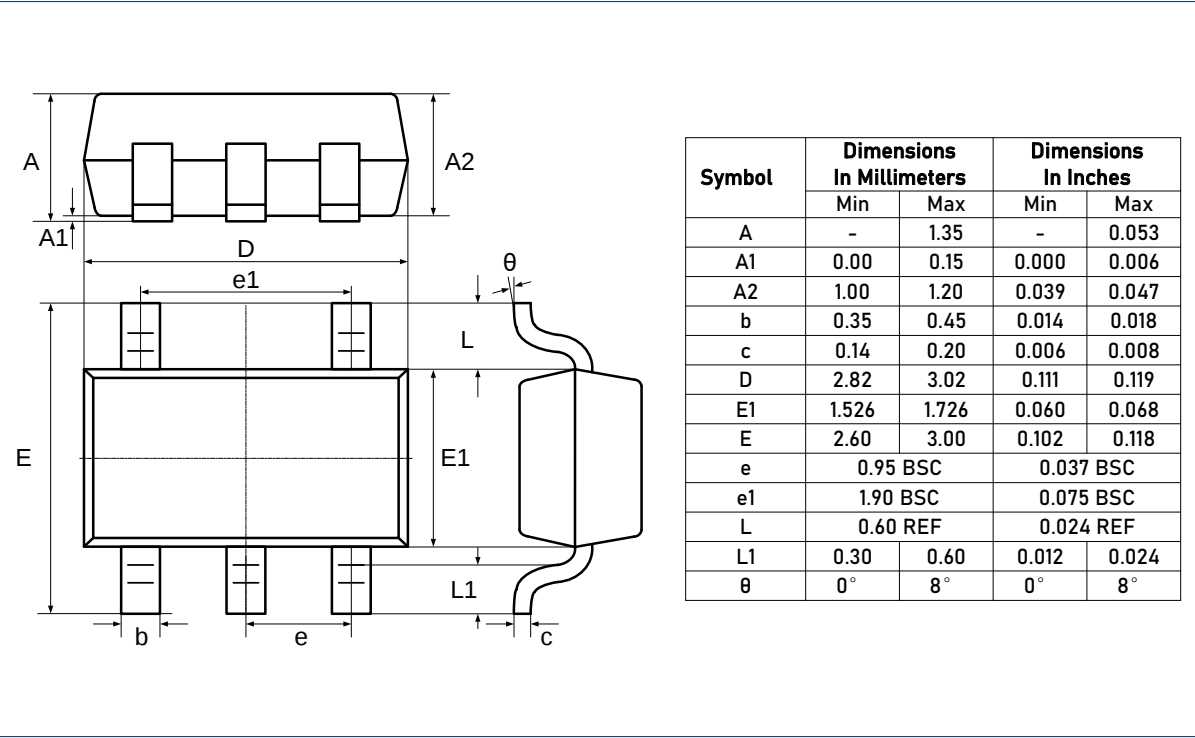
DIMENSIONS, SOT23-5L
