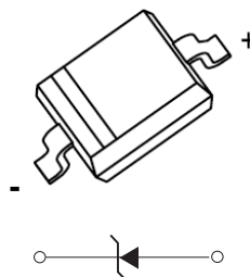
SOD-323
