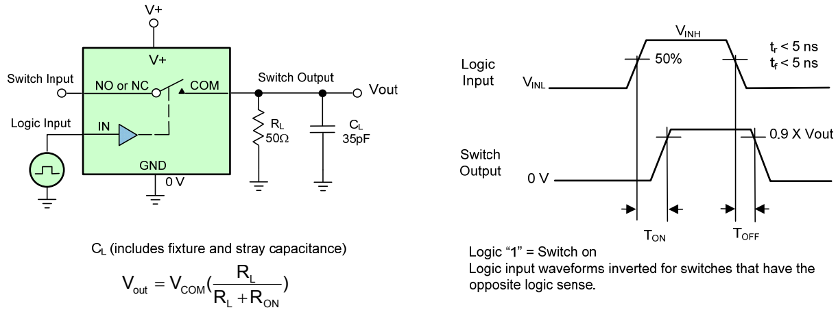
Figure 1 — Switching Time
