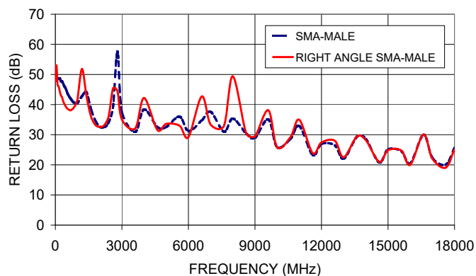
086-3SMRSM+ RETURN LOSS
