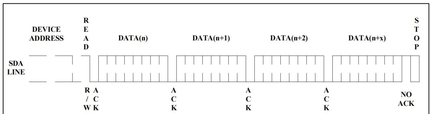
Figure 10. Sequential Read
