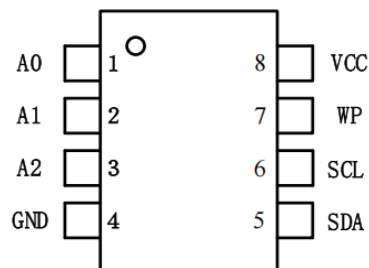
8 -lead TSSOP
