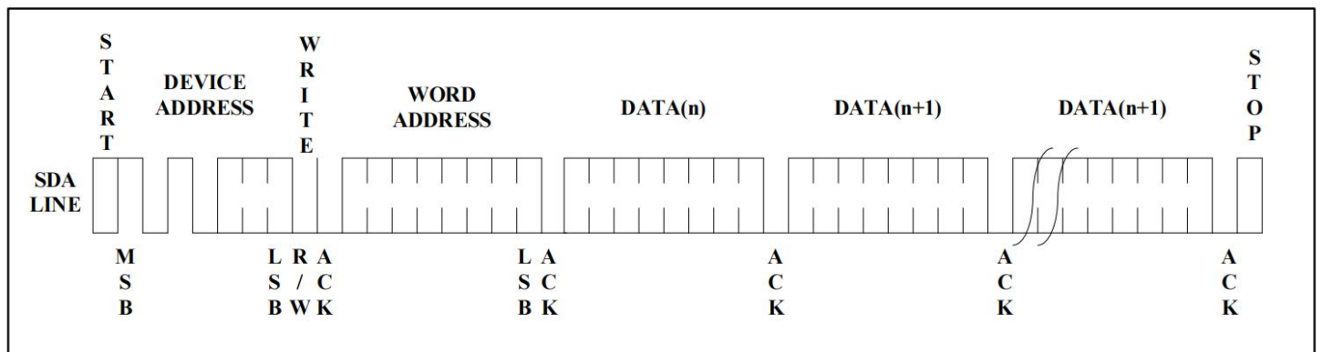
Figure 7. Page Write
