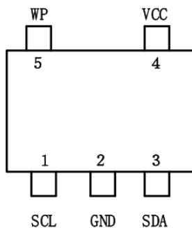
5-lead TSOT23-5
