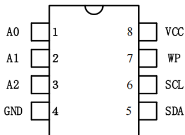
8 -lead PDIP
