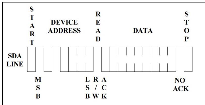
Figure 9. Random Read
