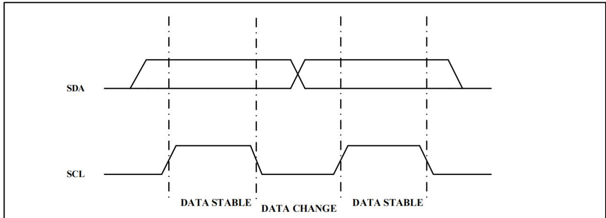
Figure 2. Data Validity
