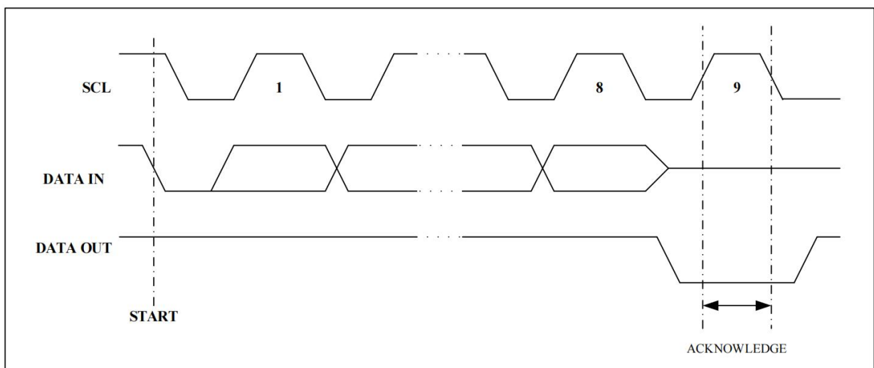
Figure 4. Output Acknowledge
