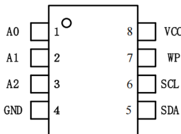
8 -lead SOP
