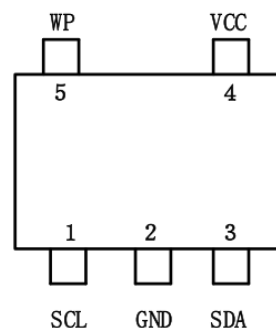
5-lead SOT23-5
