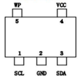
5-lead SOT23-5
