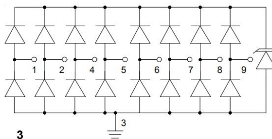
Circuit Diagram
