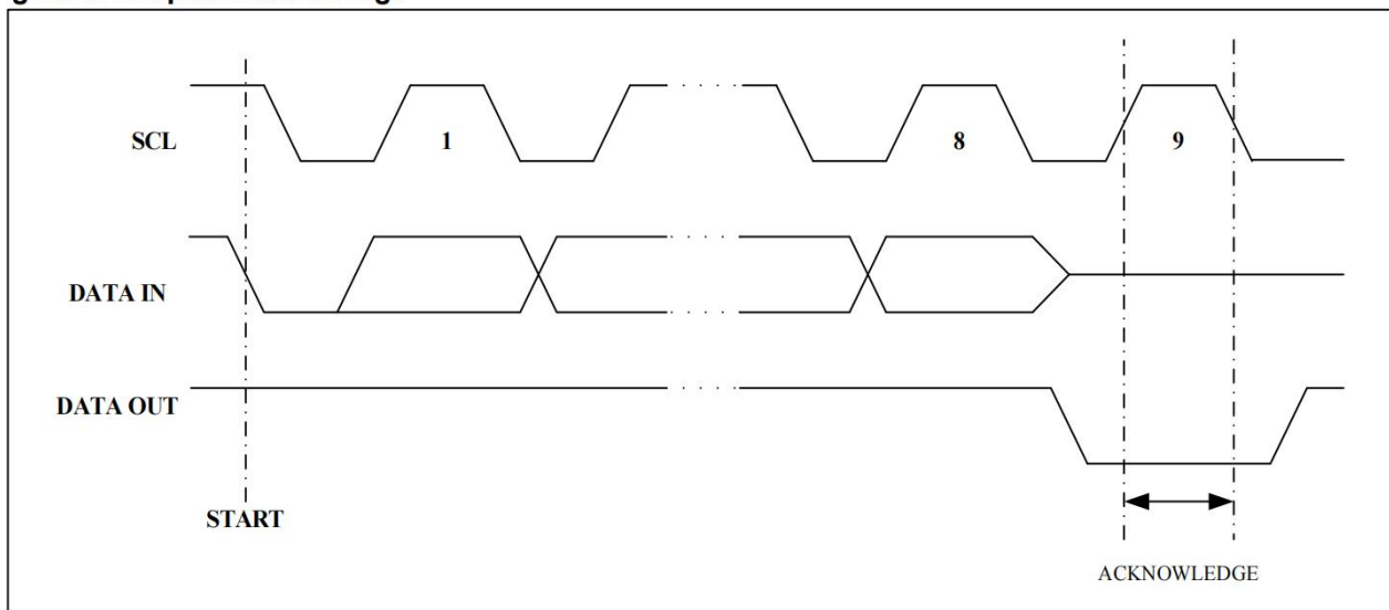
Figure 3. Output Acknowledge
