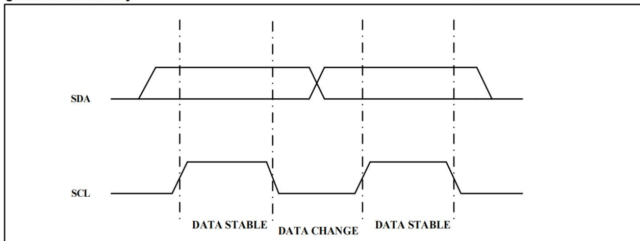
Figure 1. Data Validity
