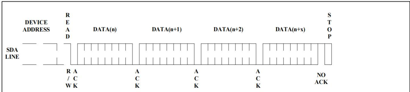
Figure 9: Sequential Read
