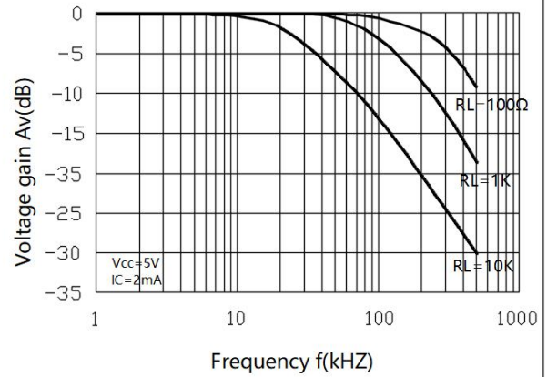
Fig.8 Frequency Response
