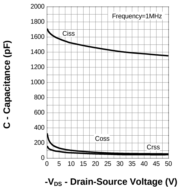
Capacitance
