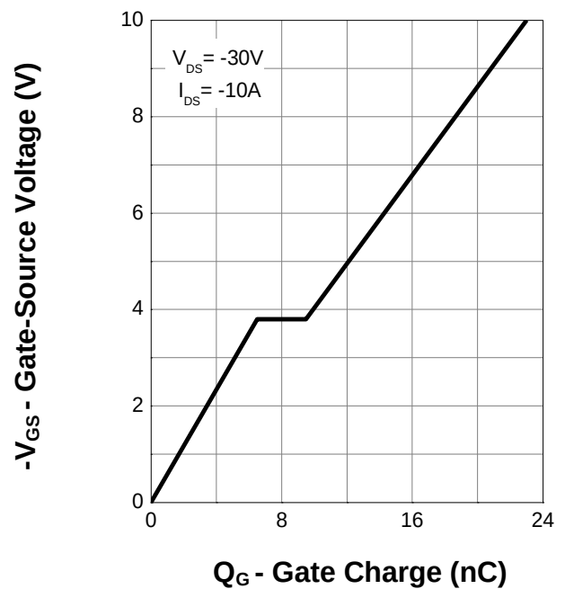
Gate Charge
