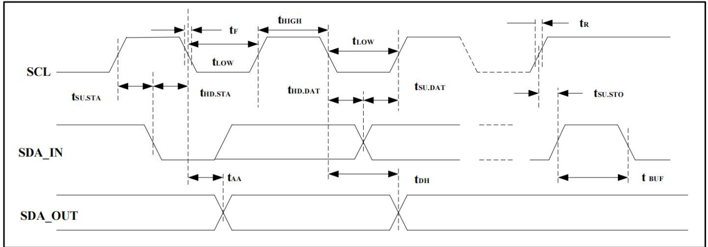
Figure 10: SCL: Serial Clock, SDA: Serial Data I/O
