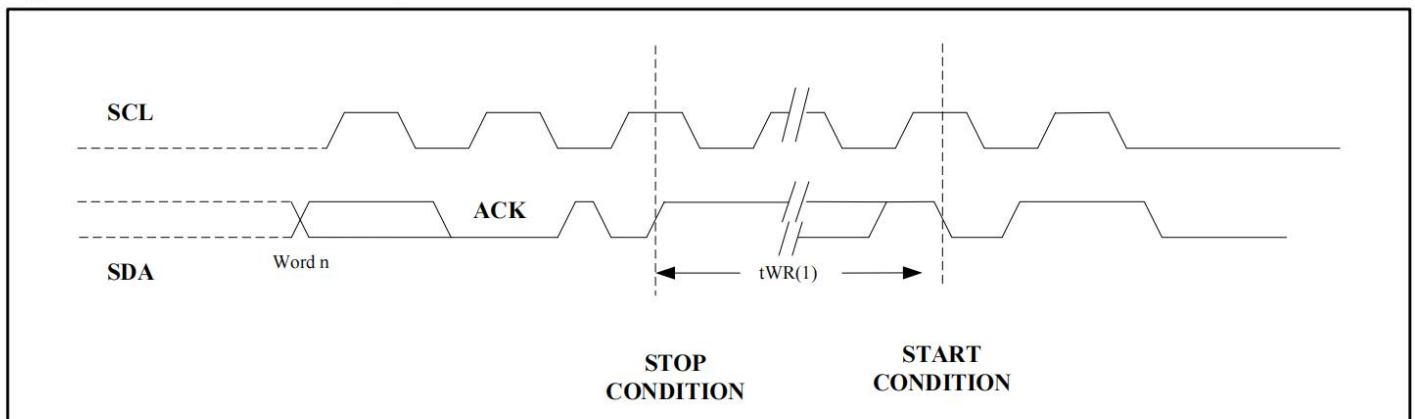
Figure 11: SCL: Serial Clock, SDA: Serial Data I/O
